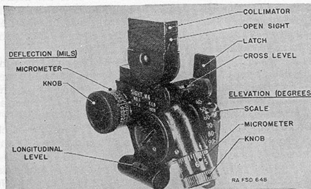
FIGURE 4.—Sight, M4.
