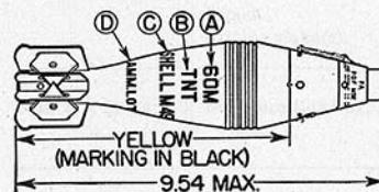
FIGURE 8.—Shell, HE, M49A1, with PDF M52.
