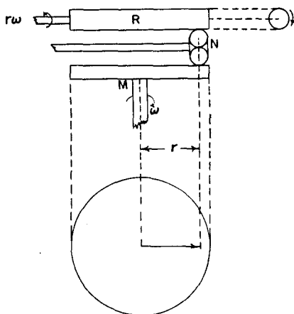
FIGURE 13.—Variable speed drive.
