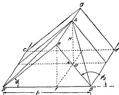
FIGURE 10.—Altimetric roof.
