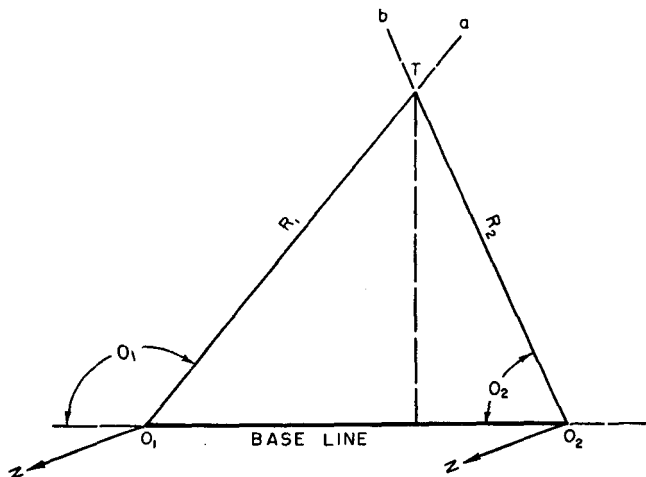
FIGURE 80.—Oblique triangle.
