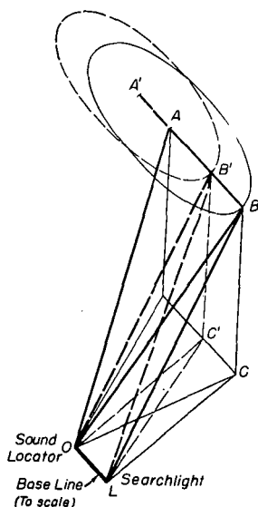
FIGURE 17.—Parallax corrections.
