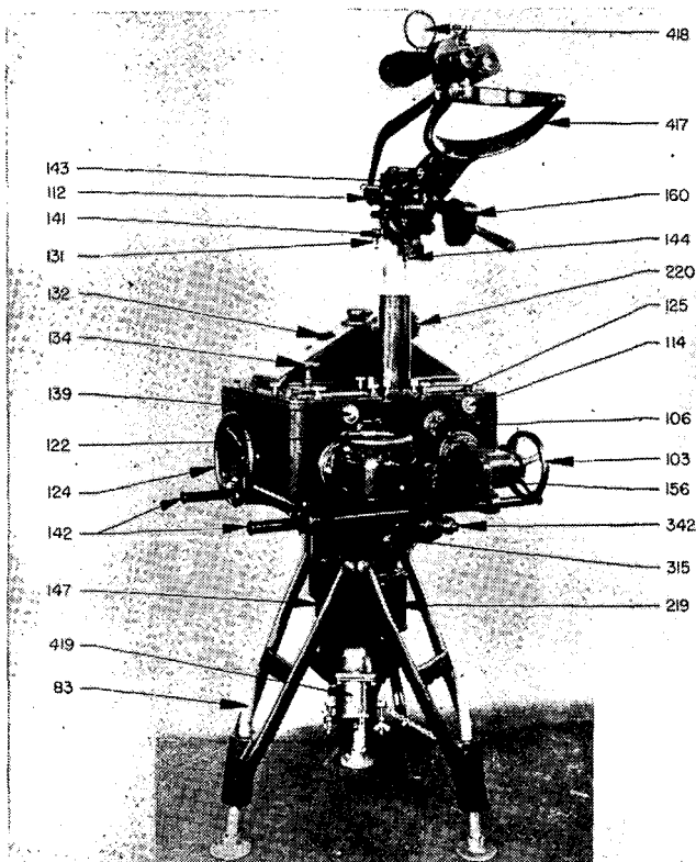
FIGURE 10.—Control station.
