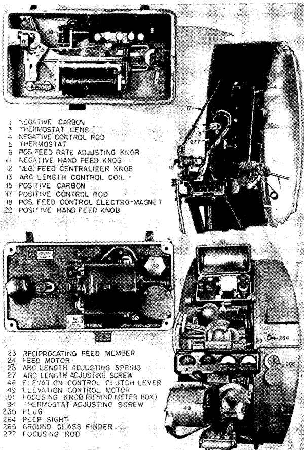
FIGURE 11.—Lamp and lamp-control mechanism.
